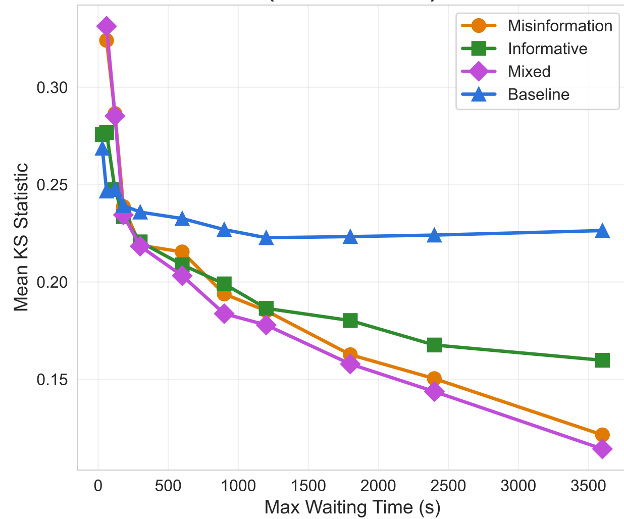
Fit Distance vs Threshold (Lower is Better)
