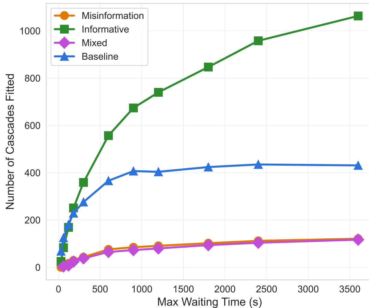
Cascade Count vs Threshold
