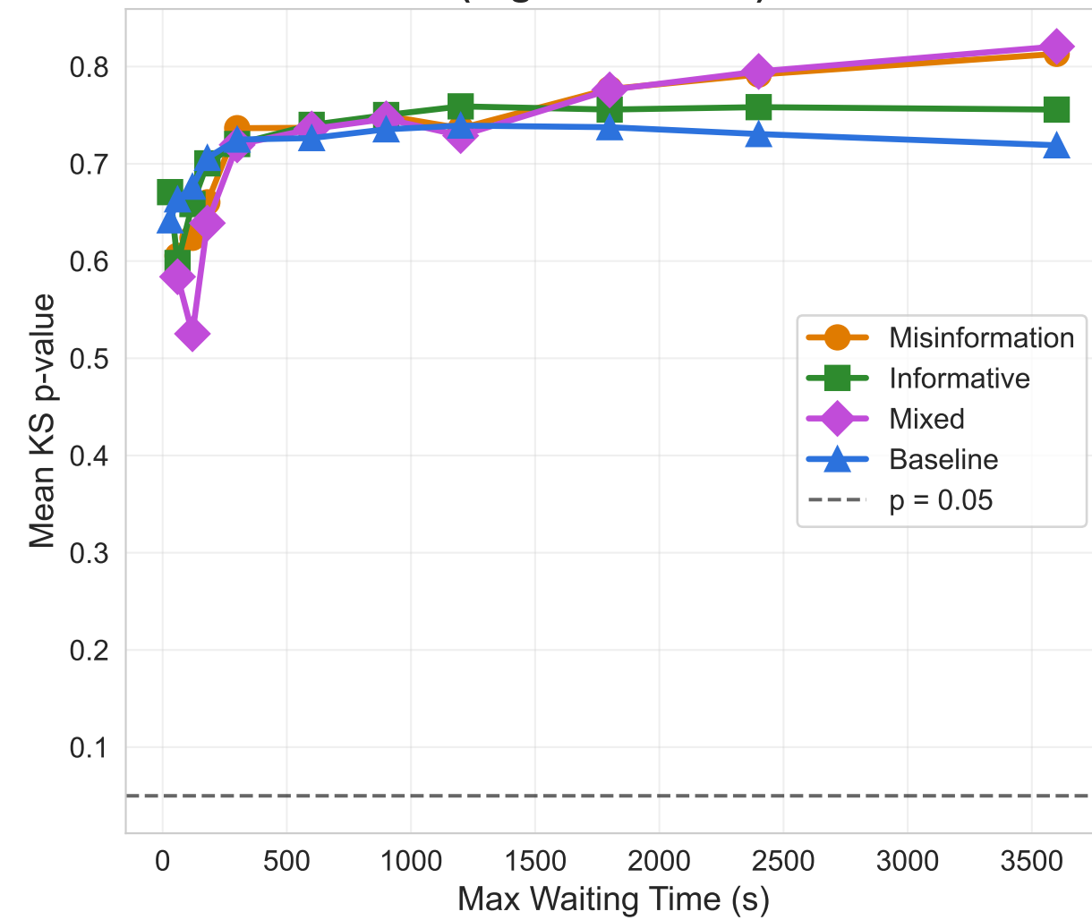
Goodness of Fit (KS test) vs Threshold (Higher is Better)
