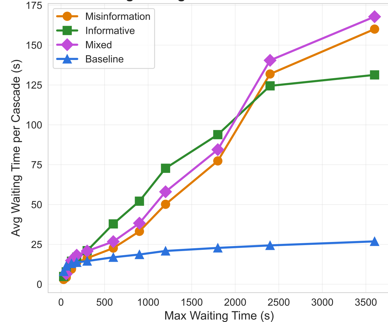
Avg Waiting Time Inside Cascades
