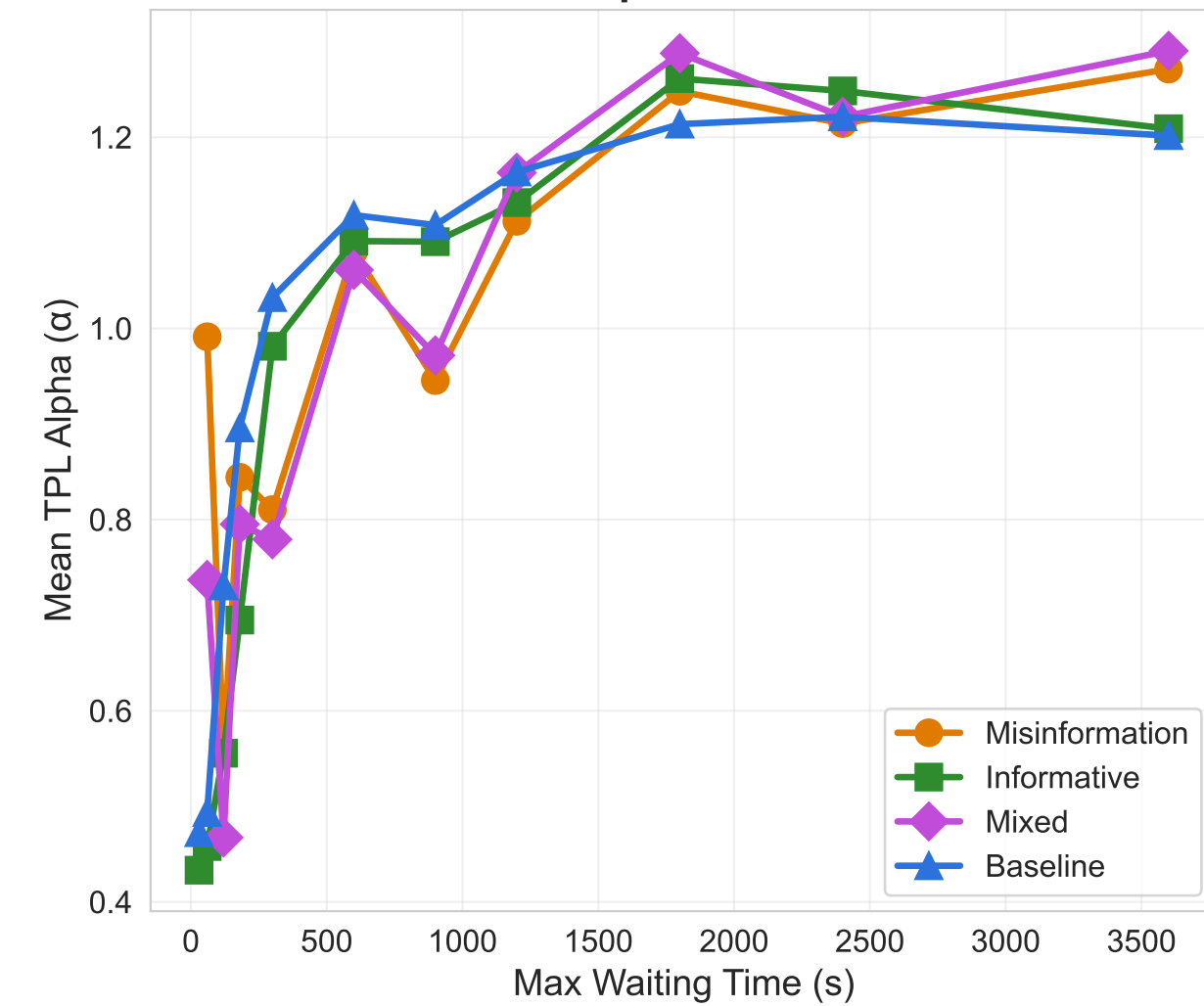
Power Law Exponent vs Threshold
